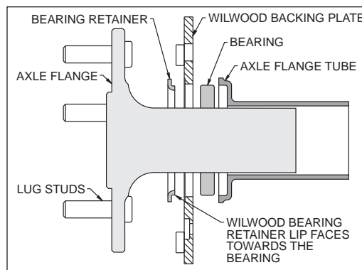
Figure 7. Retainer / Axle Diagram
