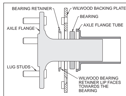
Figure 5. Retainer / Axle Diagram
