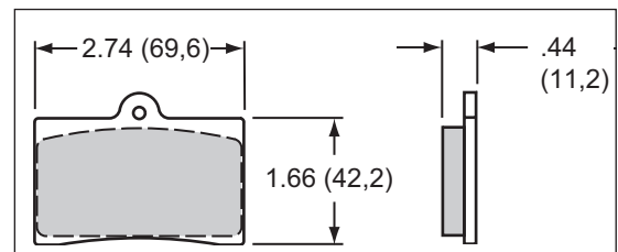
GP 320 Caliper, Type 6211 Pad Dimensions
