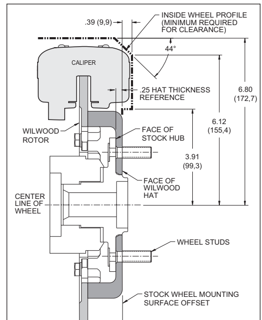
Figure 1. Wheel Clearance Diagram
