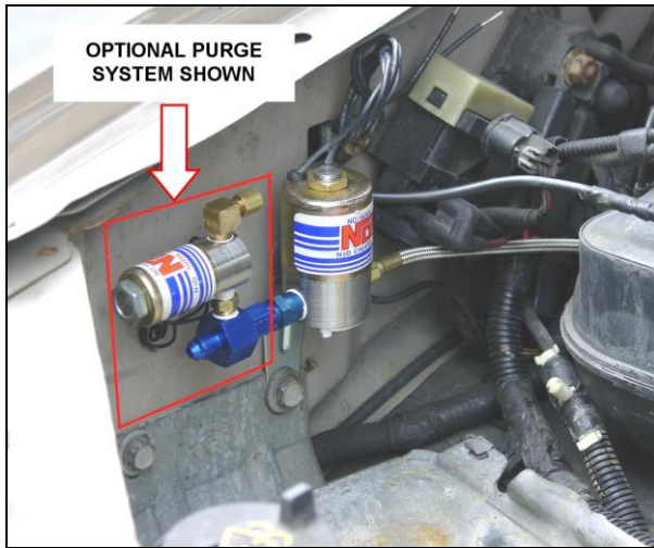
Figure 10 Mounting shown w/ optional purge
