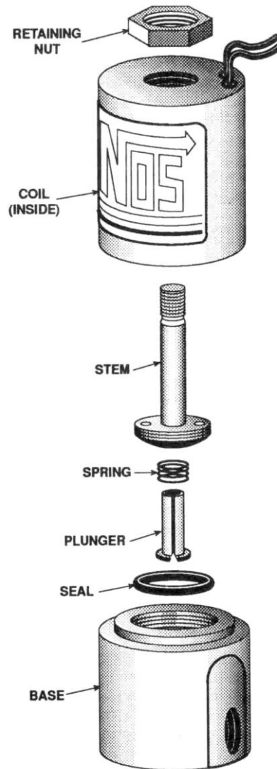
Figure 18 Exploded View of a Typical Solenoid
